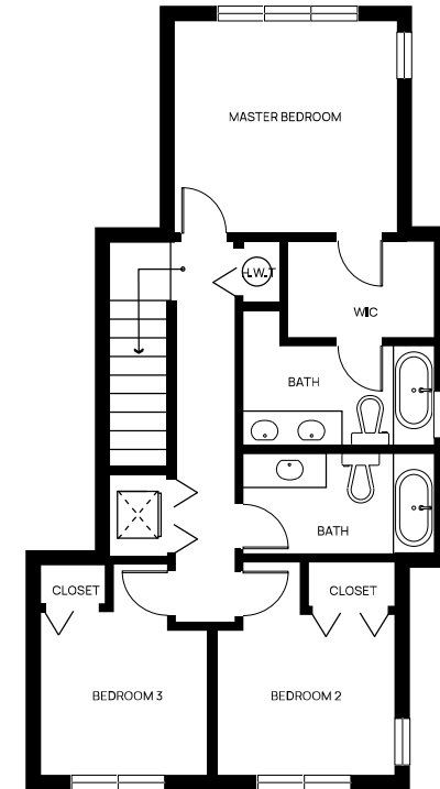
THIRD FLOOR FLOOR AREA: 660 SQ. FT.
